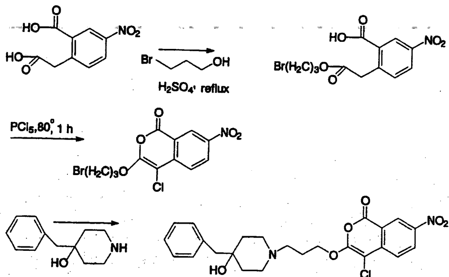
Scheme 15
